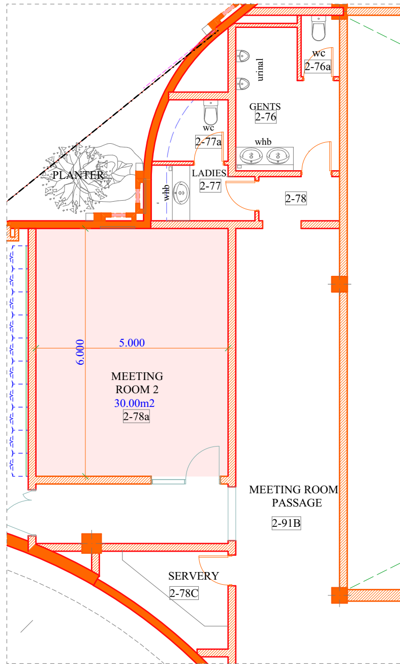
L[4]-105C New Lily Meeting Room - 1st Floor 1:100
