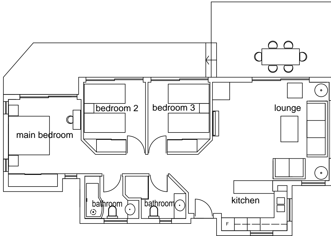
PLAN 3 BEDROOM CHALET RE6
