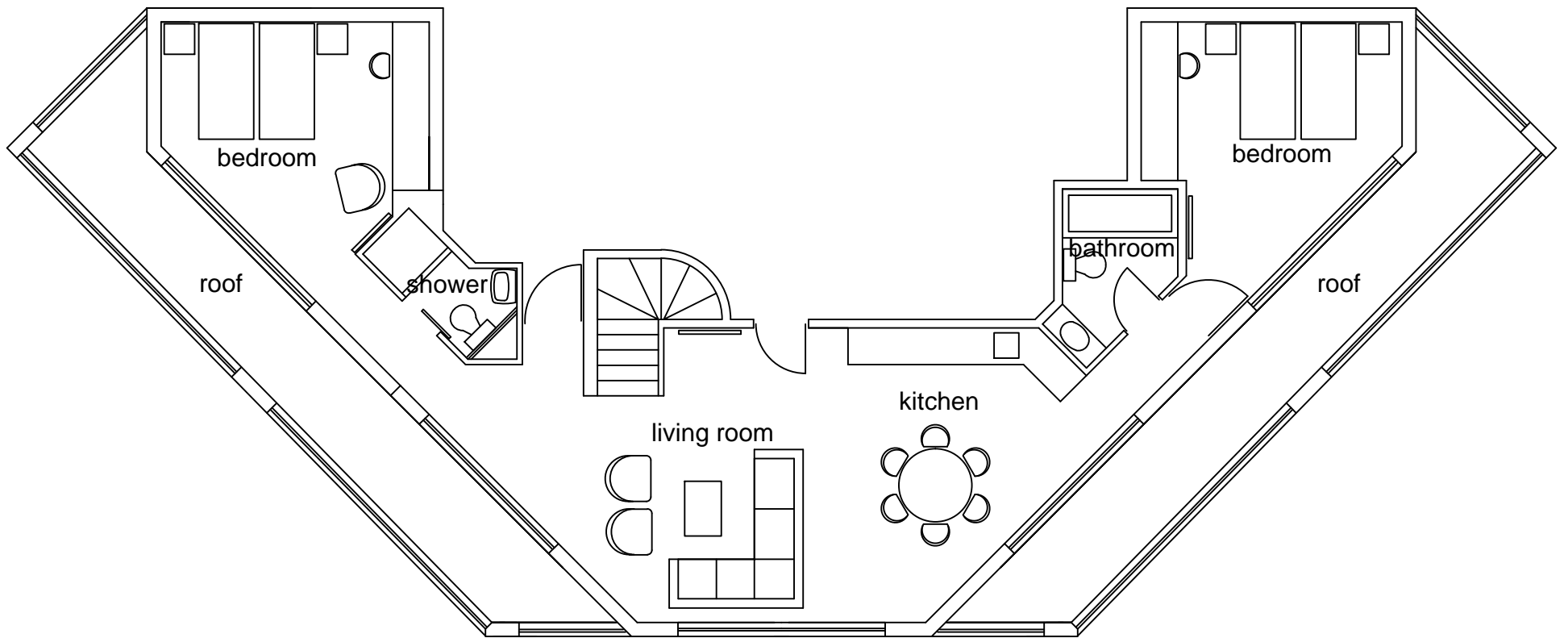
GROUND FLOOR PLAN 3 BEDROOM PENTHOUSE APARTMENT 2201
