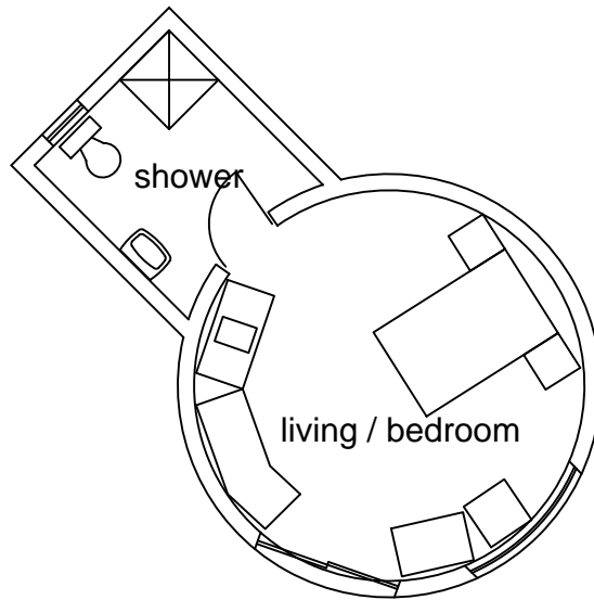
FLOOR PLAN 1 BEDROOM RONDAWEL RONDAWEL 38, 41 & 43
