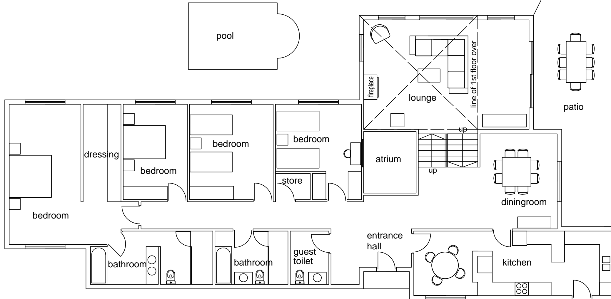
GROUND FLOOR PLAN 4 BEDROOM CHALET CHALETS - 13 & 25
