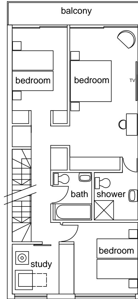
SECOND STOREY PLAN
