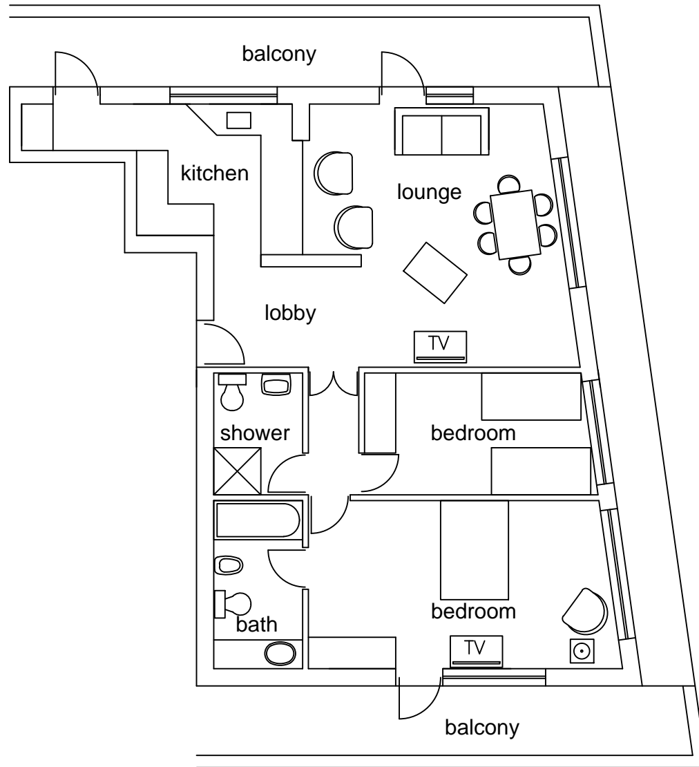
PLAN 2 BEDROOM SUPERIOR SEAVIEW APARTMENT - F1
